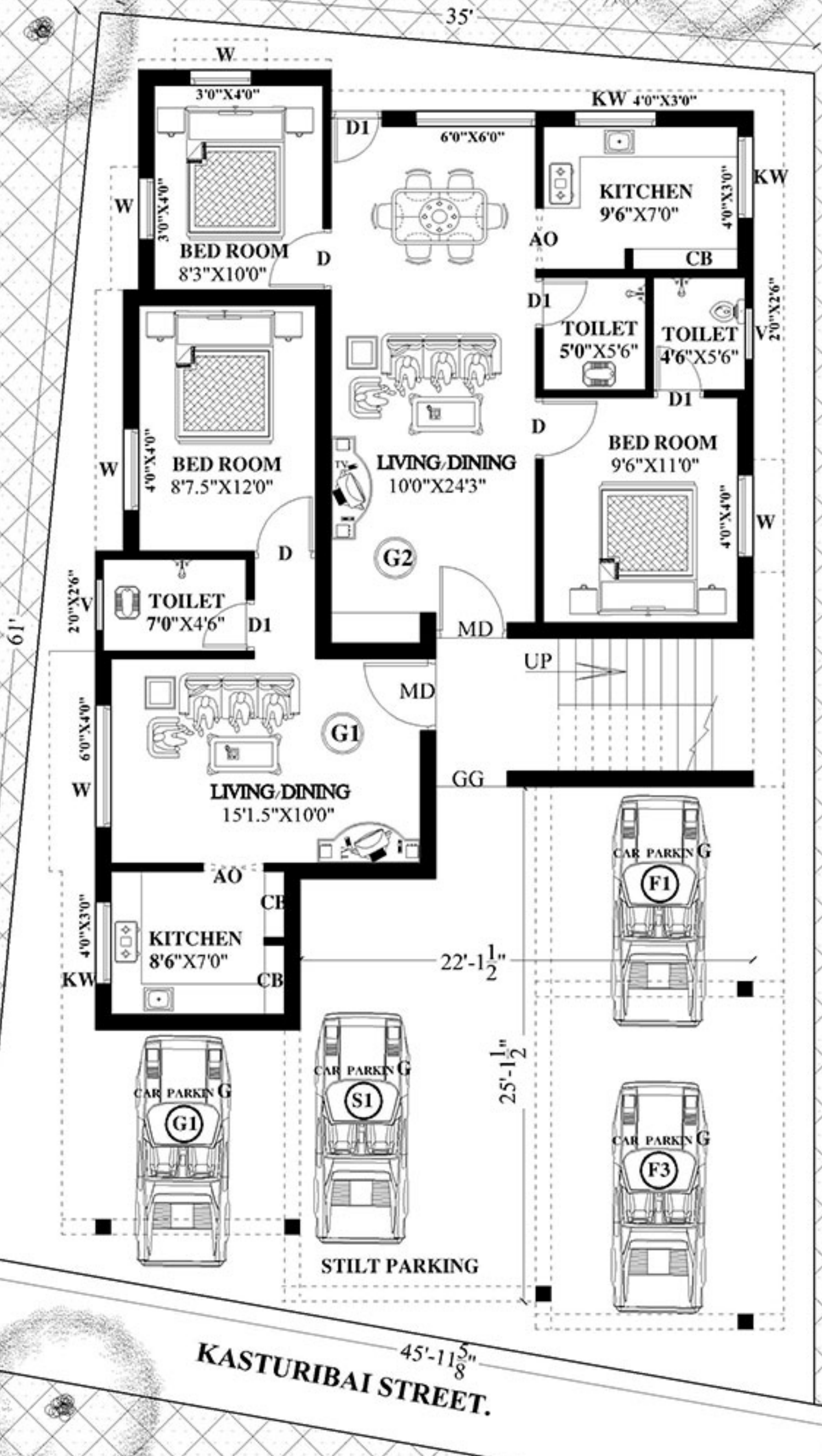
SITE CUM STILT FLOOR PLAN PART & GROUND FLOOR PLAN PART
